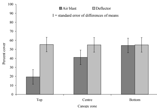
Figure 3. Improved deposition throughout the canopy using a deflector or tower
